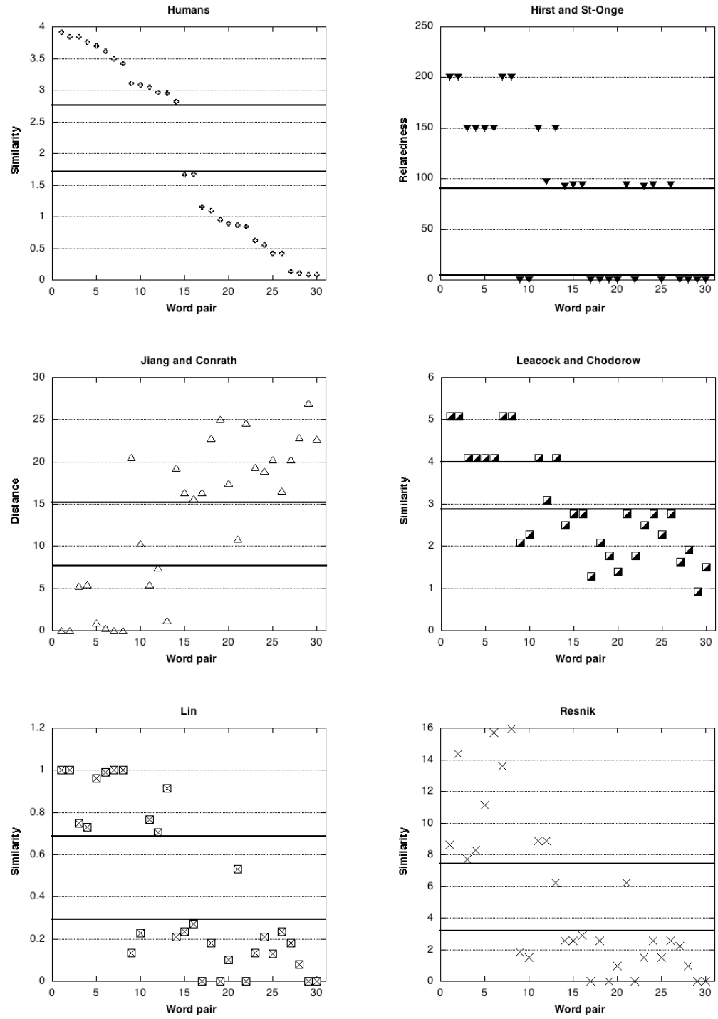
Figure 3 Human and computer ratings of the Miller–Charles set of word pairs, with sparse bands marked (see text). From left to right and top to bottom: The word pairs rated by Miller and Charles’s subjects; by the Hirst–St-Onge similarity measure; by the Jiang–Conrath distance measure; by the Leacock–Chodorow similarity measure; by the Lin similarity measure; and by the Resnik similarity measure.
