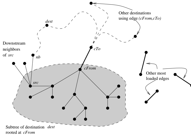
Figure 2: The search space for a move of the RSNE algorithm
