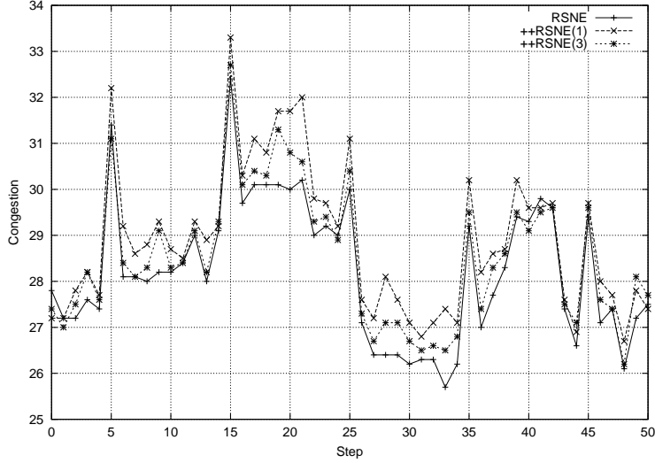
Figure 4: Comparison among RSNE and I-RSNE( k ).
