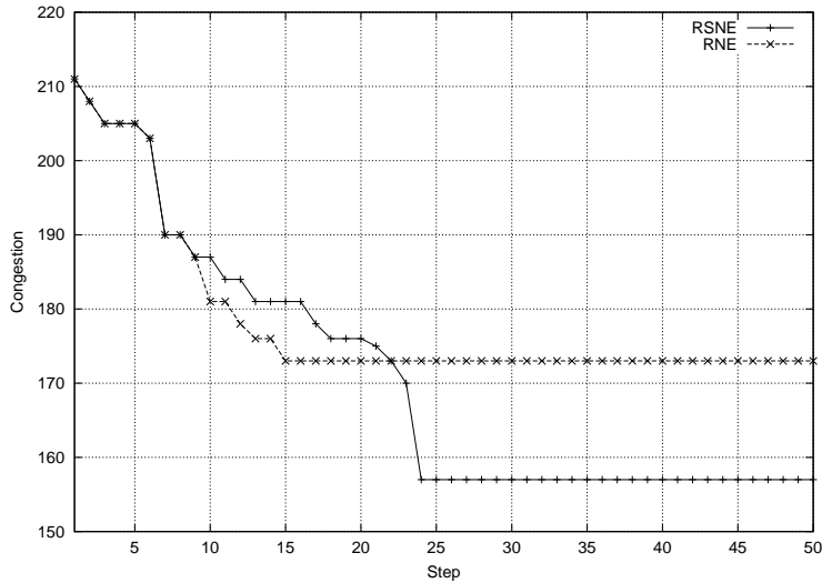
Figure 3: Comparison between RSNE and RNE algorithms.
